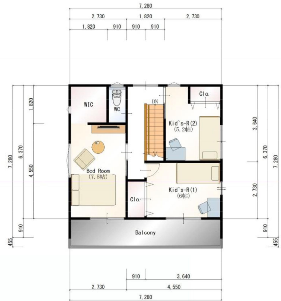
●2階 平面図
